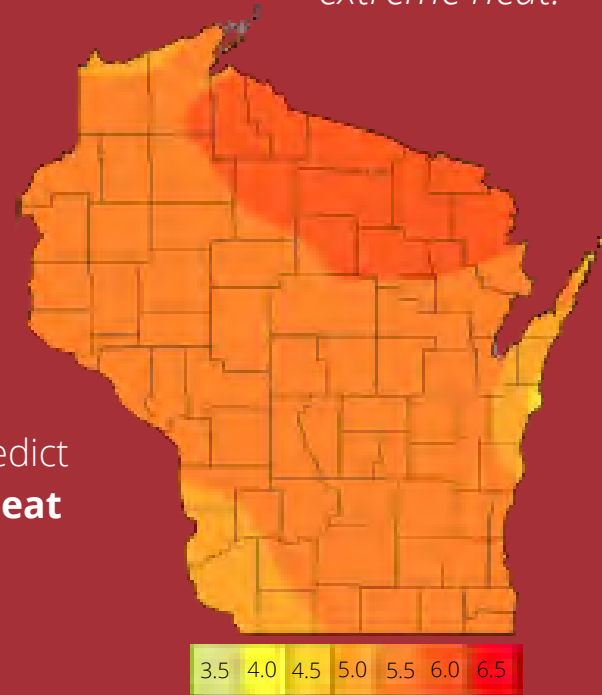
Projected Change in Summer Average Temperature (°F) from 1980-2055 22
