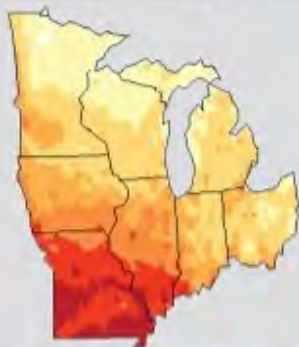
Days Above 95°F
